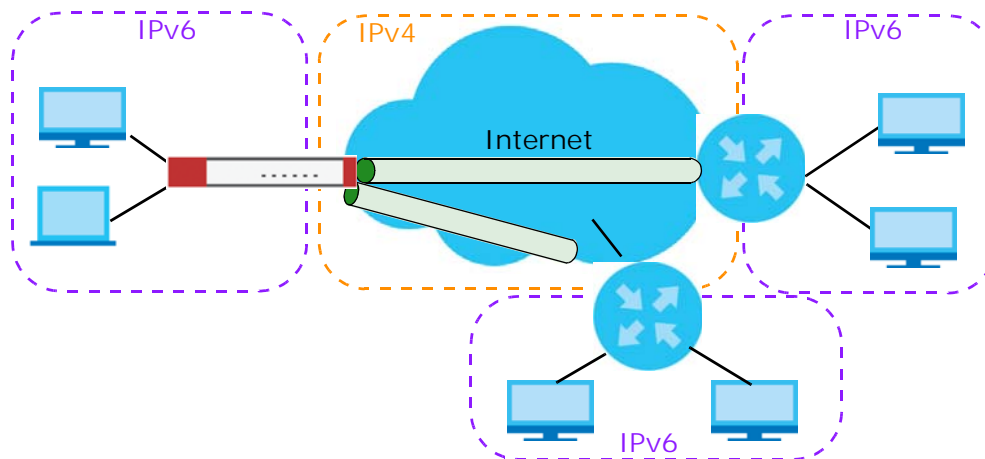
Figure 274 6to4 Tunnel
