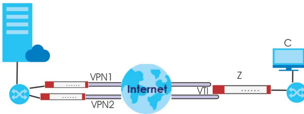
Figure 285 VTI and Trunk for VPN Load Balancing
