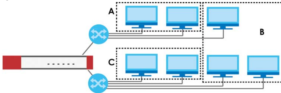
Figure 277 Example: Before VLAN
