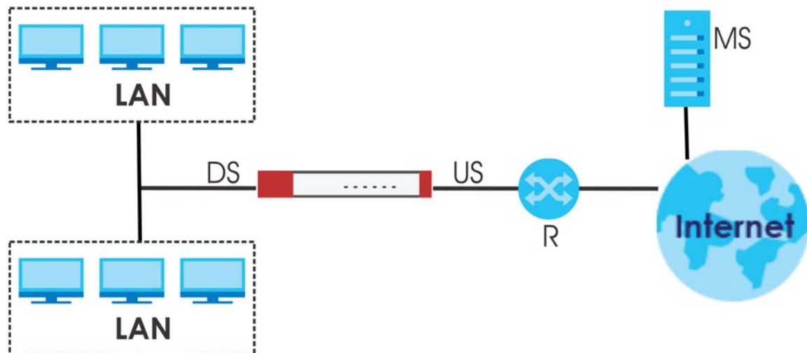
Figure 256 IGMP Proxy
